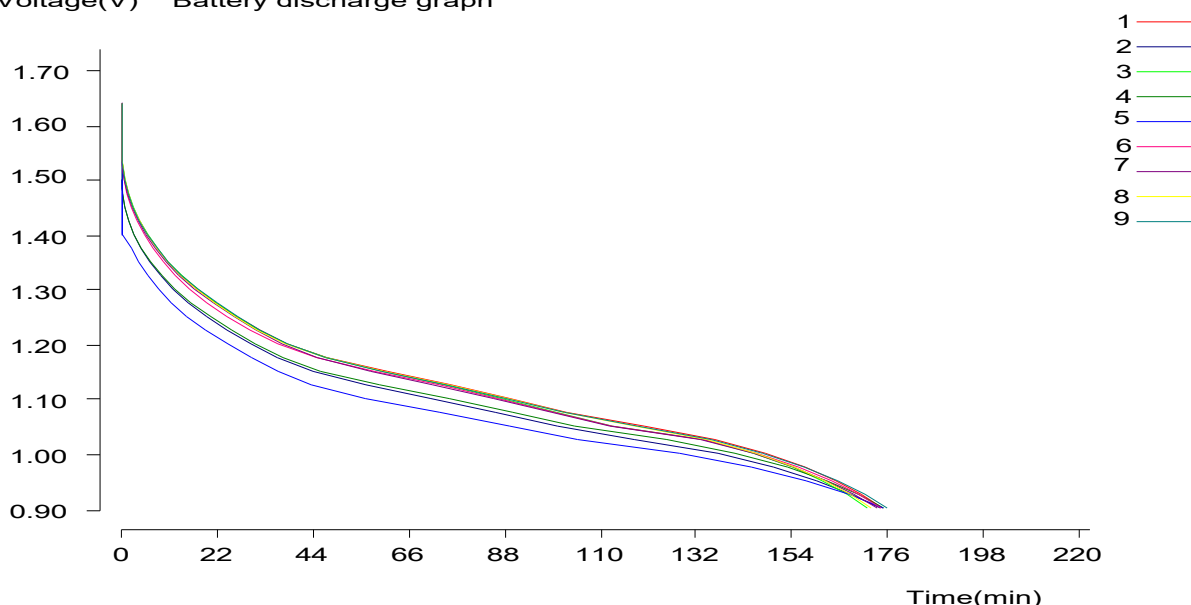
Voltage(V) Battery discharge graph
